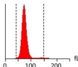
RBC Histogram
