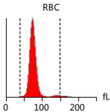
RBC Histogram
