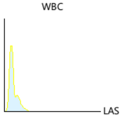
WBC Histogram
