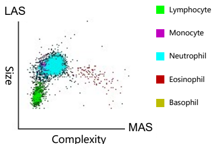
WBC Scattergram
