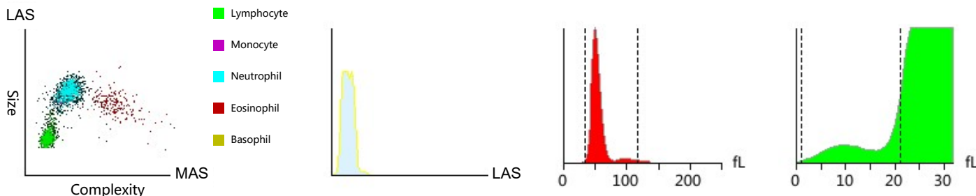
WBC Scattergram
