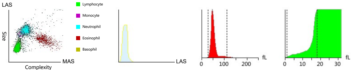
WBC Scattergram
