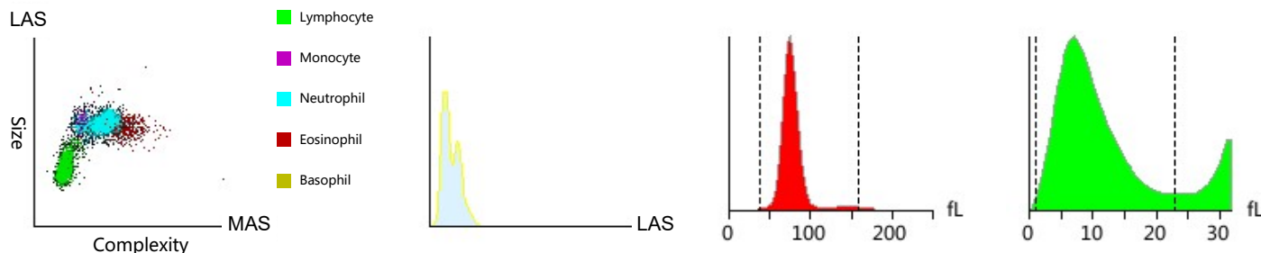
WBC Scattergram
